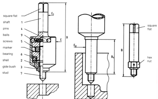
Tapper Installation Tools
